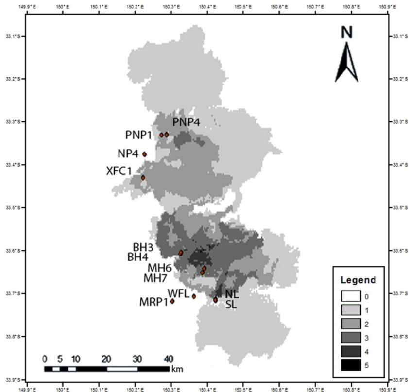
Fig. 2. Fire count (1967–2013). Raster surface of all fires impacting swamp sites showing the number of fires ('Legend') affecting those sites between 1967 and 2013 (see Table 1).
