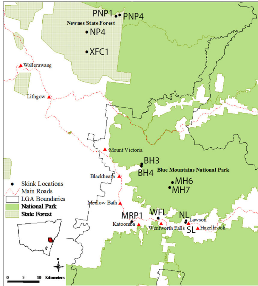
Fig. 1. Map of swamp study sites. Locations of the swamp sites within the Blue Mountains and Newnes Plateau and their land tenures (NSW NPWS 2001; see Table 1).
